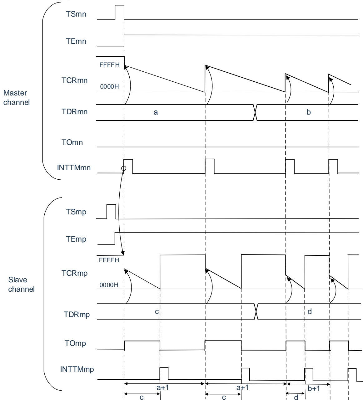
Figure 6-38: Example of basic timing operating as PWM function
