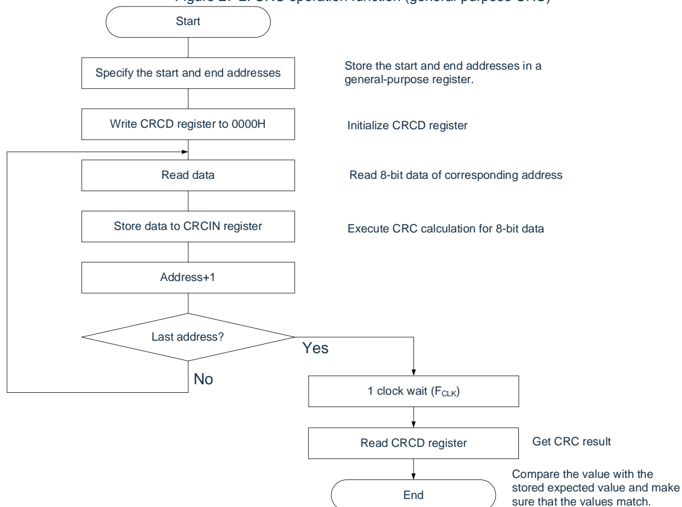
Figure 27-2: CRC operation function (general-purpose CRC)
