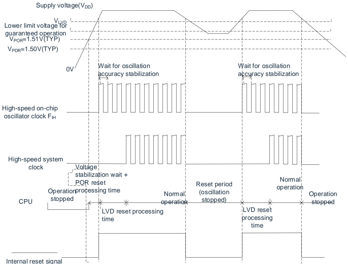
Figure 25-2: Timing of internal reset signal generation for power-on reset circuit and voltage detection circuit (3/3)
