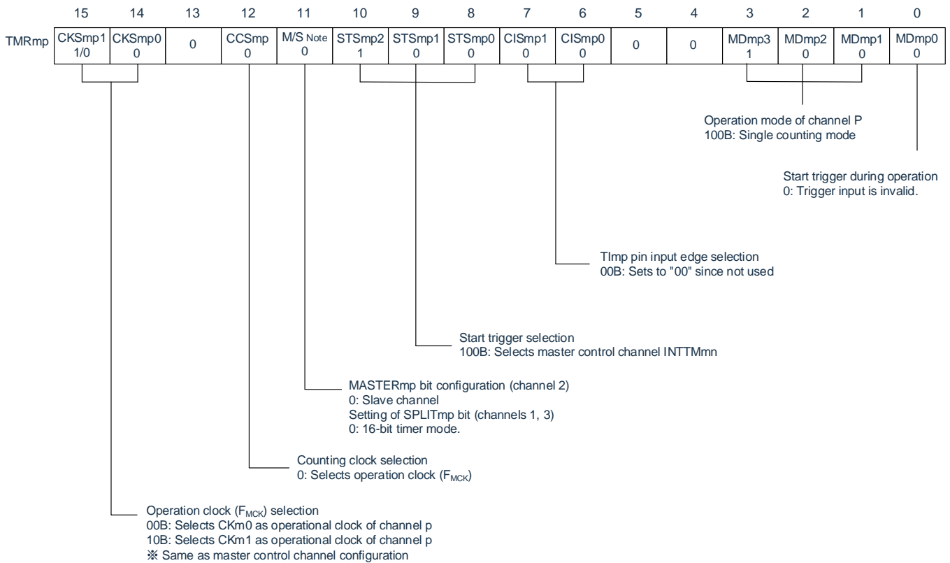
Figure 6-35: Example of register contents setting for single trigger pulse output function (slave channel)
