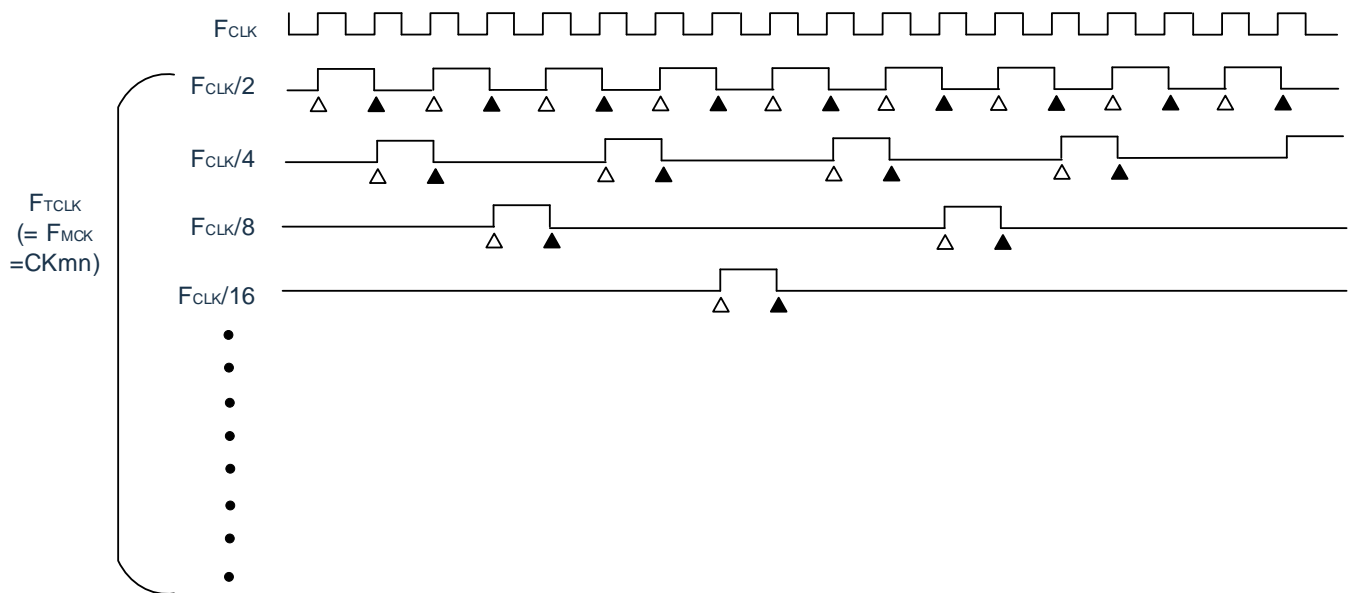
Figure 6-2: Timing of F_{CLK} and count clock ( F_{TCLK} ) (When CCSmn = 0)
