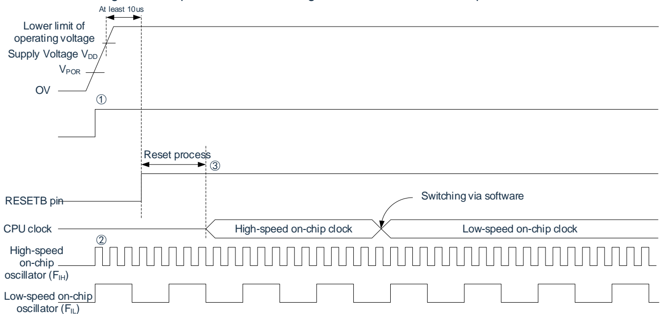
Figure 5-2: Operation of the clock generation circuit when the power is turned on
