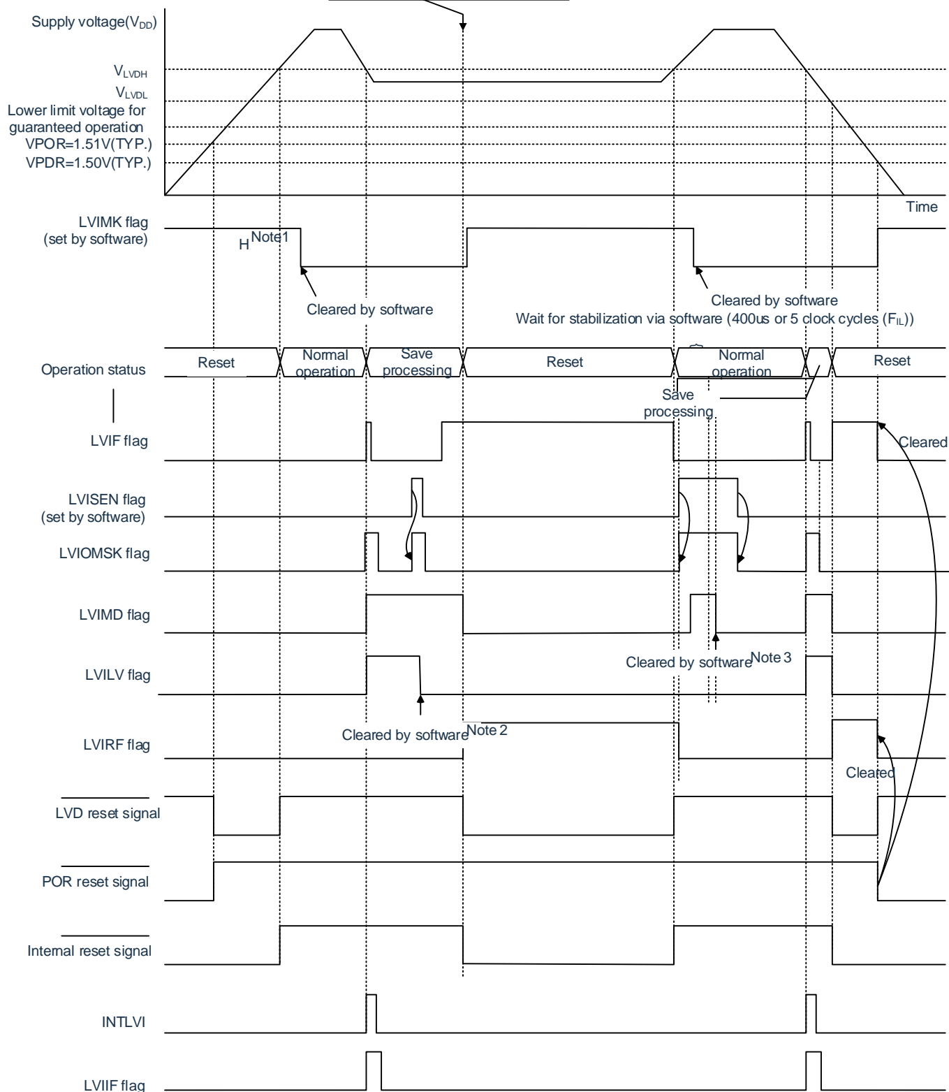
When a condition of V_{DD} is V_{DD} < V_{LVIH} after releasing the mask, a reset is generated because of LVIMD = 1 (reset mode).
