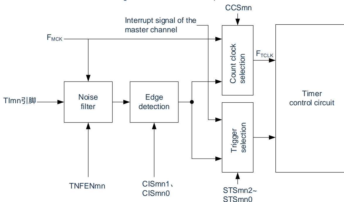
Figure 6-17: Structure of input circuit
