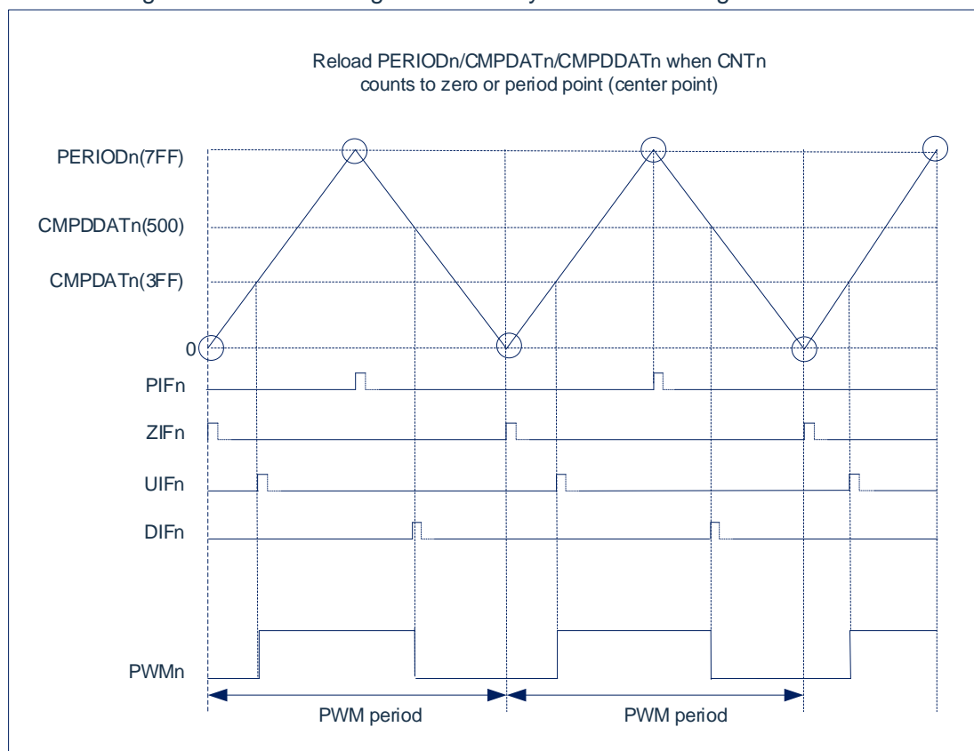
Figure 13-6: Center-aligned mode asymmetric counting waveform
