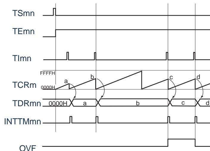
Figure 6-26: Example of basic timing operating as an input pulse interval measurement (MDmn0=0)
