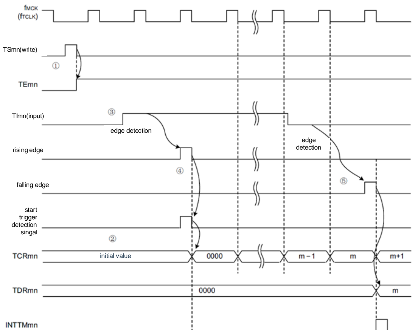
Figure 6-8: Operation timing (capture & single count mode: measurement of high-level width)
