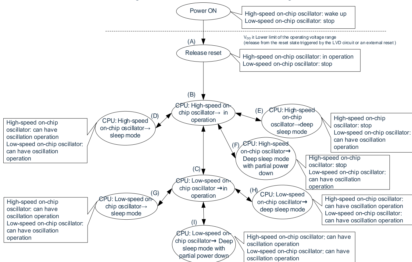
Figure 5-3: CPU clock status transition diagram
