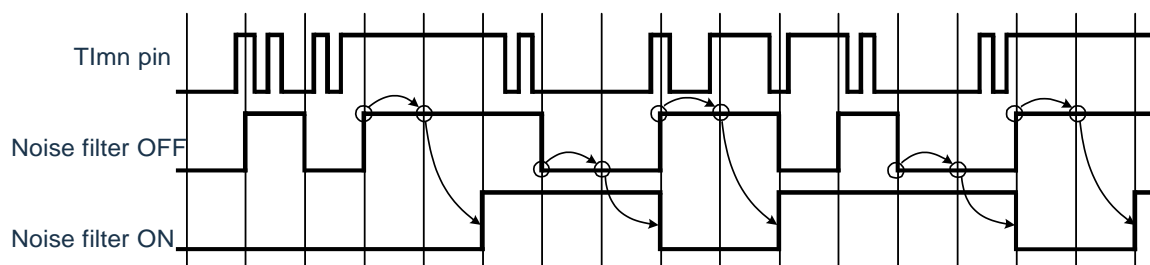
Figure 6-18: Sample waveform of Tlmn input pin with noise filter ON or OFF
