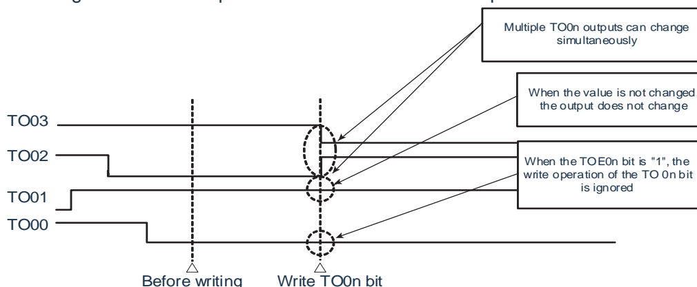
Figure 6-15: TOn pin state when the TOn bit is operated at one time
