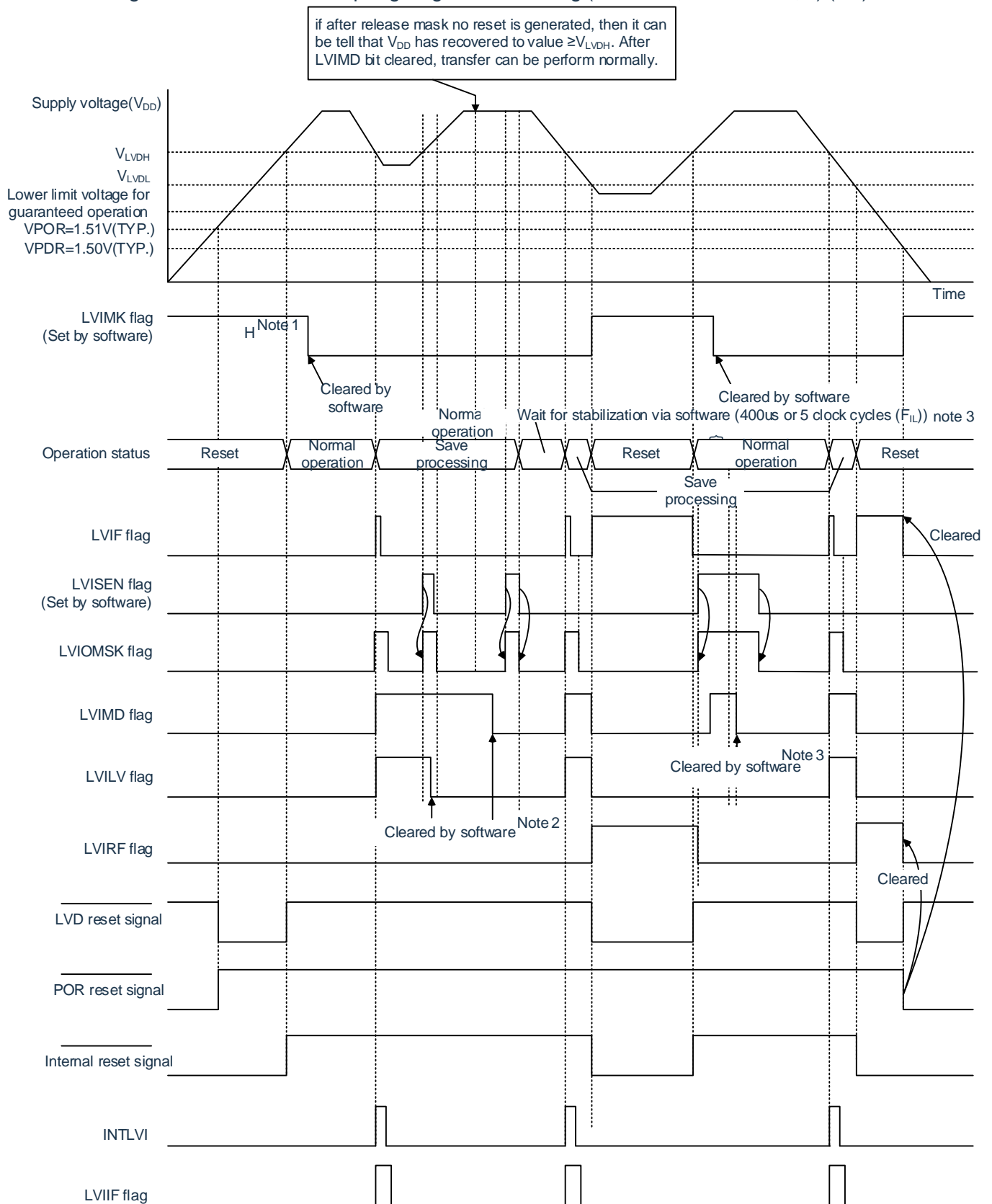
Figure 26-4: Reset &amp; interrupt signal generation timing (LVIMDS1, LVIMDS0=1, 0) (1/2)
