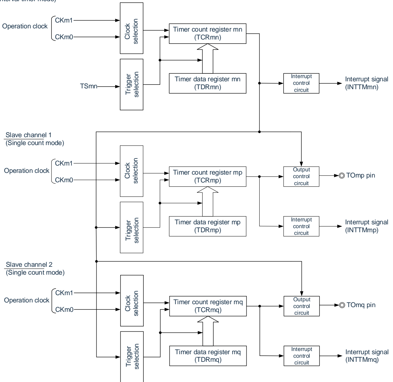
Figure 6-40: Block diagram of operation as multiple PWM output function (output two types of PWMs)
